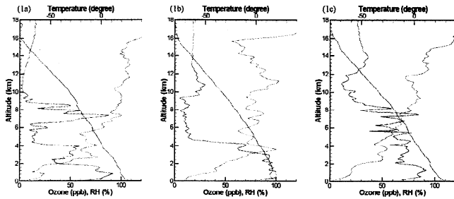
Figure 1. Ozone (red line), temperature (dark line) and relative humidity (blue line) profiles on (a) April 8, (b) 14 and (c) 21, 1994.
